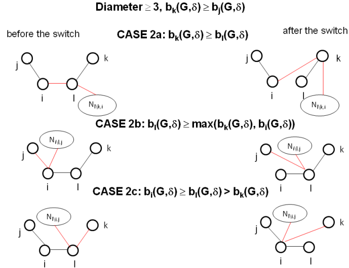
Figure 17: An N-switch preserving connectedness: diameter greater than 2
