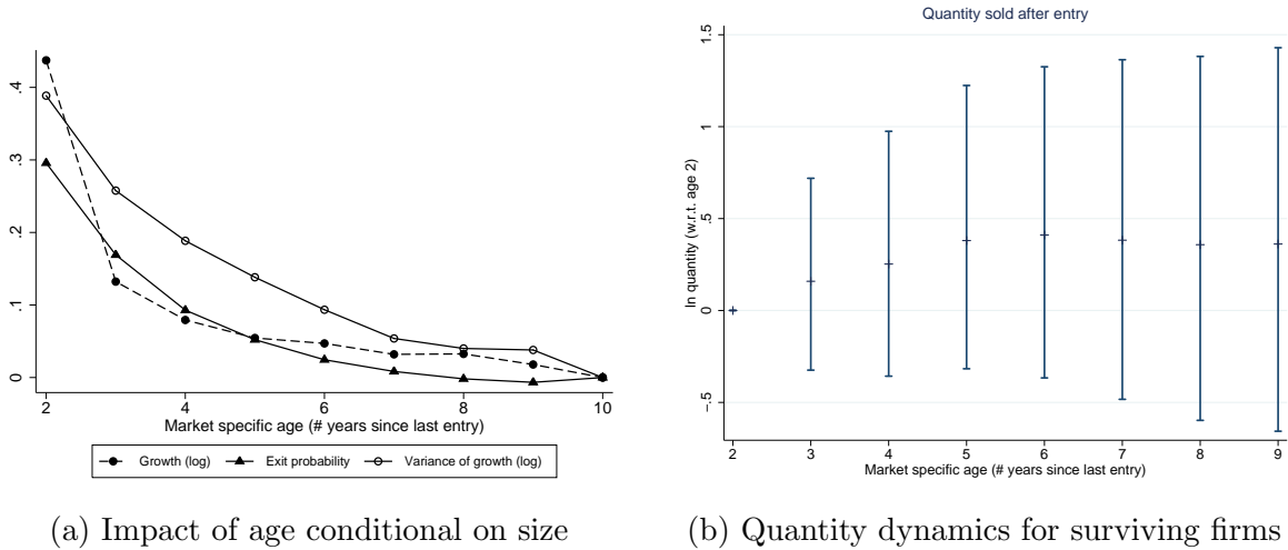
Figure 1: Stylized facts
