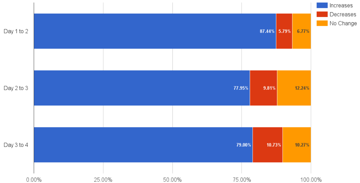
FIGURE 2.1. Proportion of programs where the cutoff values increased, decreased or did not change from one day to the next
