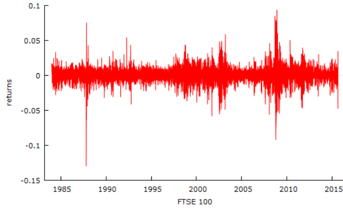
Figure 1: Daily returns series from S&P 500 (US), Nikkei 225 (JP), FTSE 100 (UK) indices. The sample is from 01-January-1984 to 31-August-2015 for days at which all the three markets were open.
