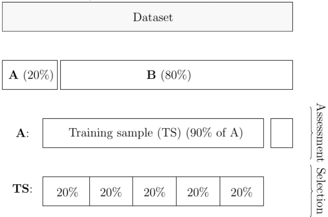
Fig. A1. Double cross-validation procedure
